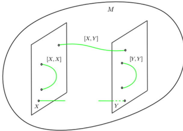
Fig.1. Geometric presentation of the category of D-branes associated to a target manifold M
